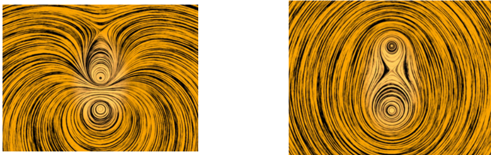
Figure 1.4.6 A flow with two circulation centers with (a) opposite directions of circulation. (b) the same direction of circulation
