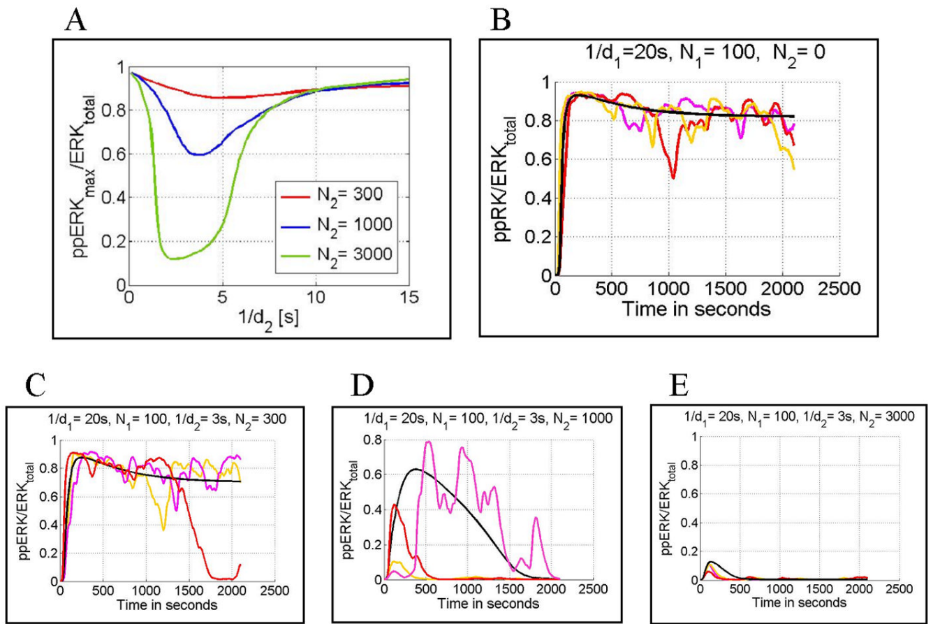
Fig. 6. Antagonism. Panel A: normalized peak ERK activity ( ppERK_{max}/ERK_{total} ) for N_1 = 100 (number of agonist peptides) and d_1 = 0.05/s (agonist peptide dissociation rate constant) as a function of 1/d_2 (inverse antagonist peptide dissociation rate constant). The red, blue and green lines correspond to N_2 = 300, 1000, 3000 (number of antagonist peptides). Panels B through E: normalized ppERK(t) calculated for N_1 = 100, d_1 = 0.05/s, d_2 = 0.333/s and N_2 = 0, 300, 1000, 3000 , respectively. The black line is obtained from a deterministic simulation, whereas the red, pink, and yellow lines are obtained from stochastic simulations. In all cases, peptide stimulation started at t_i = 0 s and lasted for t_s = 2100 s.
