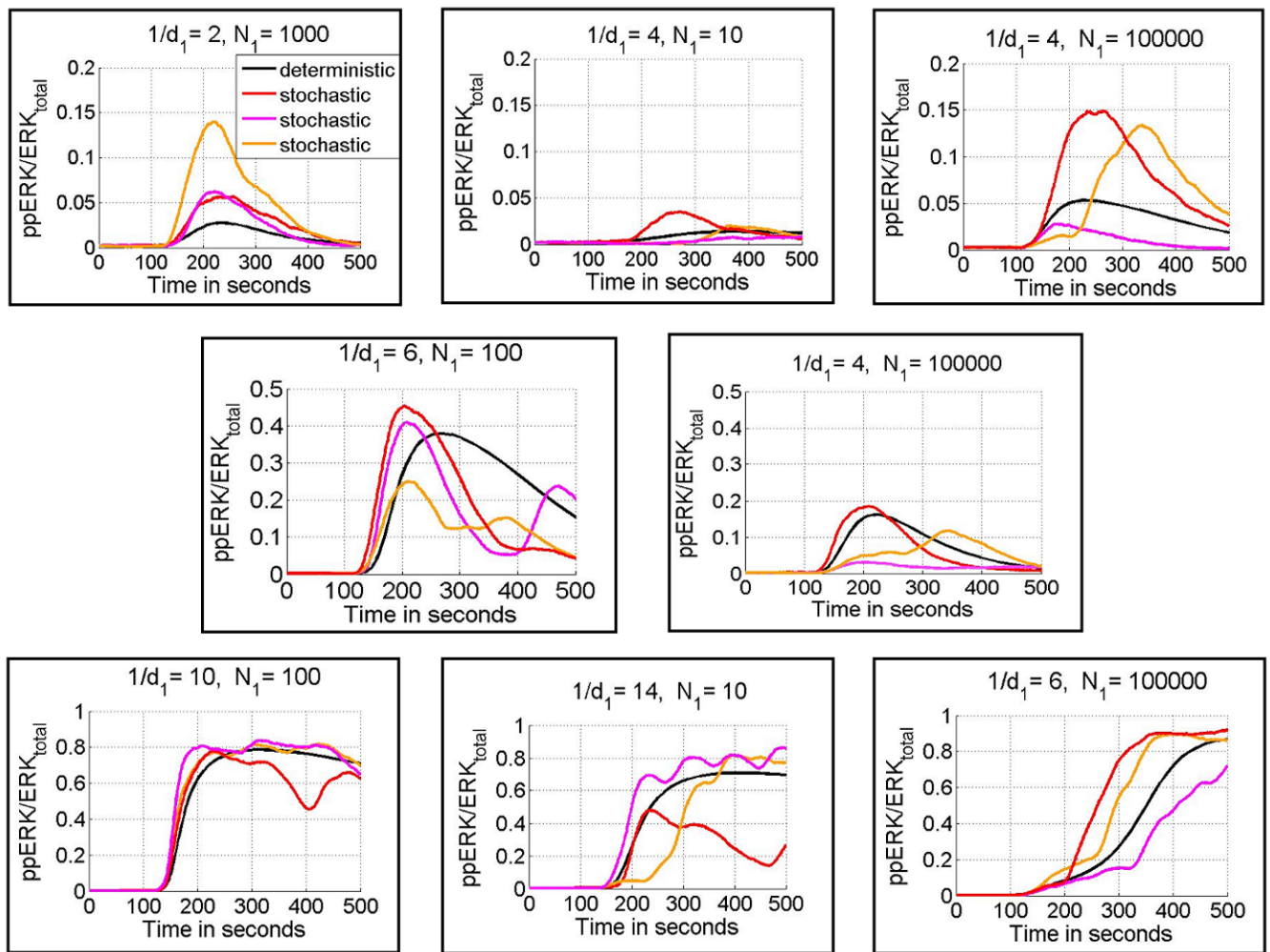
Fig. 4. ppERK(t)/ERK_{total} calculated in deterministic (black-line) and stochastic (red, pink and orange) simulations, for eight points in (1/d, \log(N)) parameter space shown in Fig. 3. Panels in upper, middle, and lower rows correspond, respectively to points from low, intermediate and high ERK activity domains indicated in Fig. 3. Notice the different vertical scale for each row. Peptide stimulation started at t_i = 100 s (from the beginning of the numerical simulation) and lasted for t_s = 400 s.
