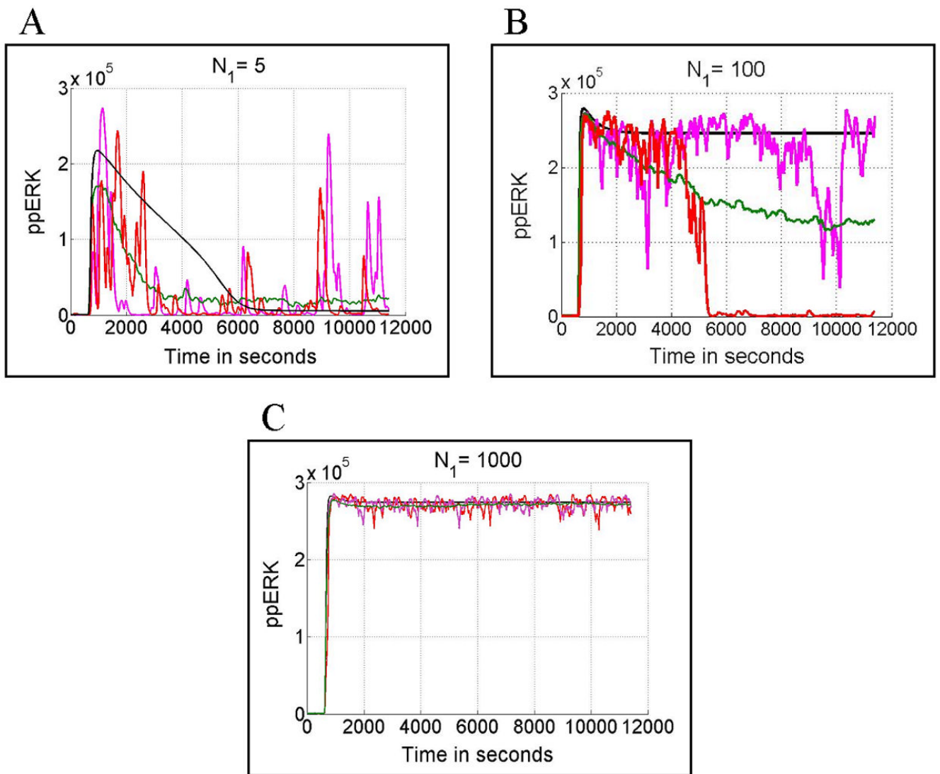
Fig. 8. ppERK( t ) calculated in deterministic (black line) and stochastic (red and pink lines) simulations, for d_1 = 0.05/s and, respectively for N_1 = 5 (Panel A), N_1 = 100 (Panel B) and N_1 = 1000 (Panel C). The green line is the average over 100 stochastic simulations. In all cases cells are initially in a primed state (low levels of ppERK and pSHP). Peptide stimulation started t_i = 10 min. and lasted for t_s = 3 hour.
