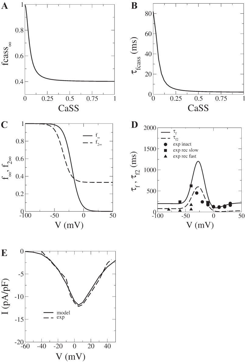
Fig. 3. A : steady-state subspace calcium inactivation ( f_{\text{CaSS}} ) curve. B : time constant curve of subspace calcium inactivation ( \tau_{\text{CaSS}} ). C : steady-state curves of slow ( f_{\infty} ) and fast ( f_{2\infty} ) voltage inactivation. D : time constant curves of slow ( \tau_f ) and fast ( \tau_{f2} ) voltage inactivation. Experimental (exp) time constants are added for comparison and are taken from Beuckelmann et al. (5), Benitah et al. (3), Mewes et al. (36), Sun et al. (58), Li et al. (32), Pelzmann et al. (46), and Magyar et al. (35). Experimental inactivation time constants represent the slowest time scale of calcium current inactivation, thus corresponding to f gate inactivation. For recovery from inactivation, both fast and slow experimental time constants are available, corresponding to f_2 and f gate recovery. E : peak current-voltage relationship of the L-type calcium current as determined in simulated voltage-clamp experiments. Experimental data are from Magyar et al. (34).
